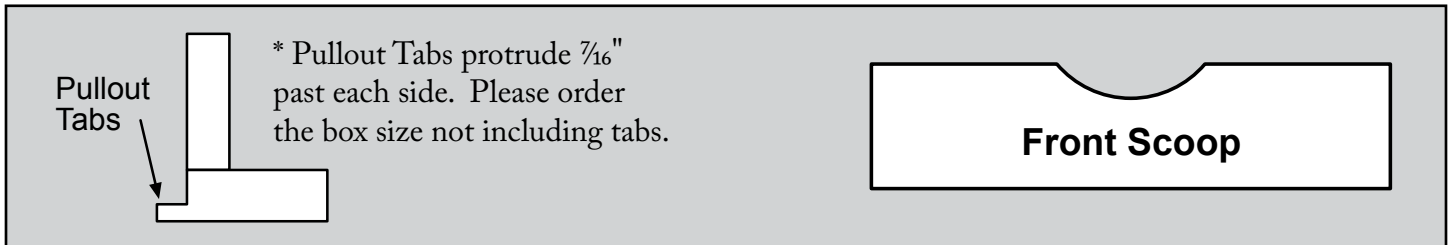
Dovetail Drawer Box
